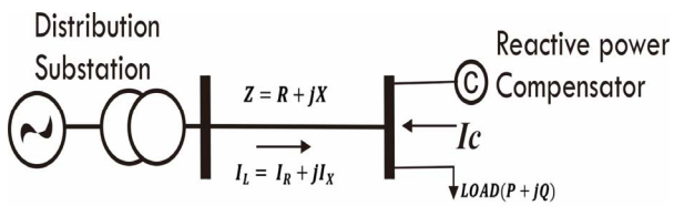
Fig. 1. Capacitor Installed in Parallel [25]
