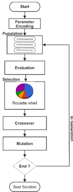
Fig. 2. Flowchart of the Genetic Algorithm Program [33]
